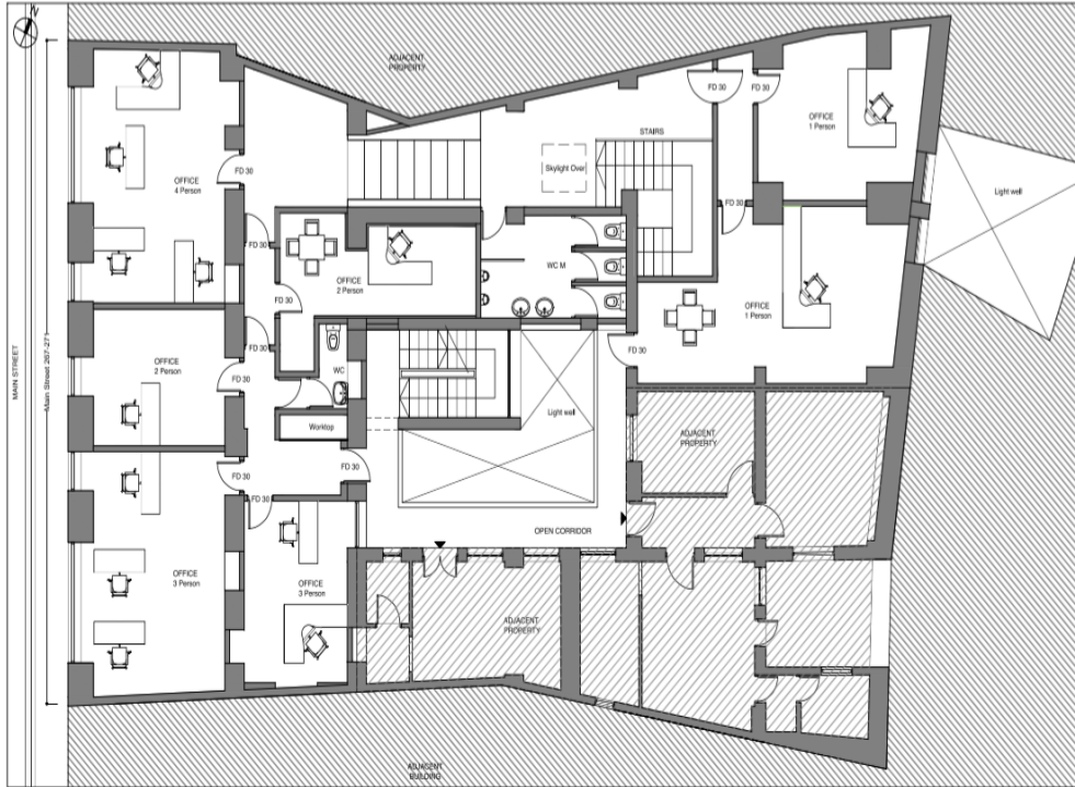
First Floor as Existing Scale 1:100
